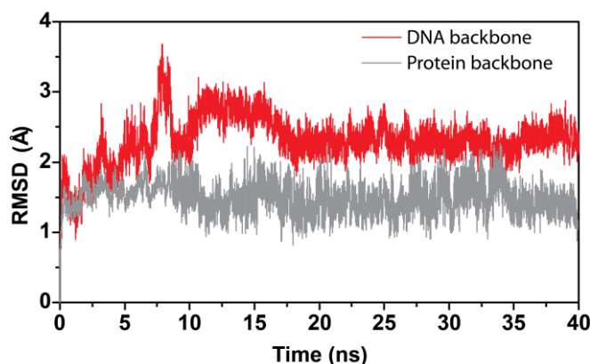
Figure S7. Root mean square deviation graphs of the trajectories obtained from MD simulation of protein and the LdG modified template and primer DNA. RMSD values from the MD trajectories were calculated with the corresponding initial structure using ptraj module in AMBER 12.
