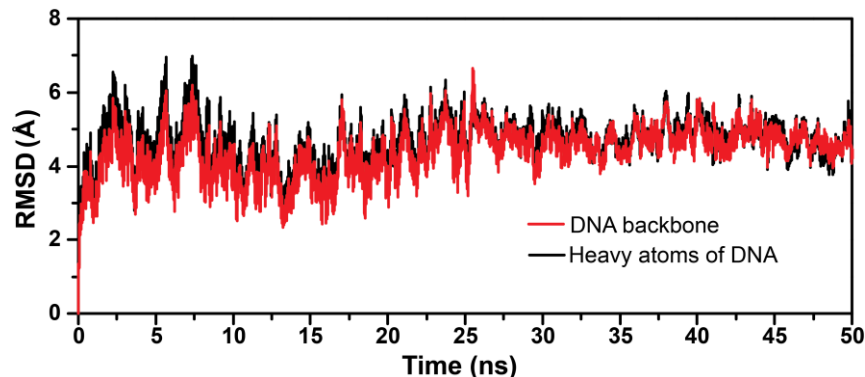
Figure S5. Root mean square deviation graphs of the trajectories obtained from MD simulation of the LdG modified duplex DNA. RMSD values from the MD trajectories were calculated with respect to the corresponding initial structure using ptraj module in AMBER 12.
