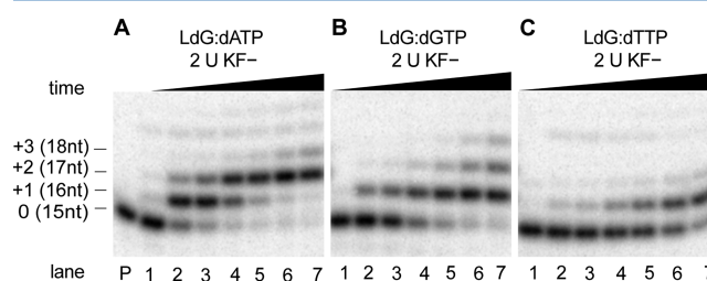
Figure 3. PAGE (20%, 7 M urea) of single nucleotide misincorporation using \text{KF}^- . The sequences of the primer and the LdG-modified template are same as in Figure 2A. (A) dATP; (B) dGTP; (C) dTTP. Lane P, primer; lanes 1 to 7, reactions for different time course from 0.5, 5, 10, 30, 60, 120, and 240 min. All the reactions were carried out at 37 ^\circ\text{C} using 2 U of \text{KF}^- in the polymerase buffer (50 mM NaCl, 10 mM Tris-HCl, 10 mM \text{MgCl}_2 , 1 mM DTT, pH 7.9).
