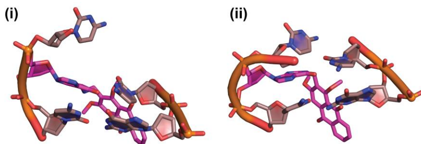
Figure S8. MD simulation snapshots around the LdG modification of template-primer DNA duplex obtained from ensemble analysis. The LdG modification is highlighted in magenta.
