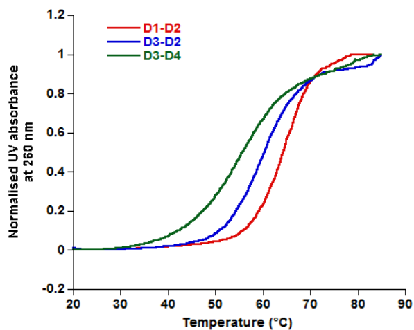
Figure S2. UV thermal melting of the unmodified and the LdG modified DNA duplexes performed using the phosphate buffer (100 mM NaCl, 20 mM phosphate buffer, 0.1 mM EDTA, pH 7.4). Melting curves were obtained using 5 \mu M concentration of ds DNA.
