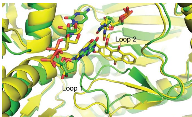
Figure S9. Superimposed structure of the Bacillus fragment (BF) in complex with the LdG modified DNA (yellow) and the unmodified DNA (green). The LdG modification (yellow) with the pairing dC and the dG with pairing dC is highlighted.
