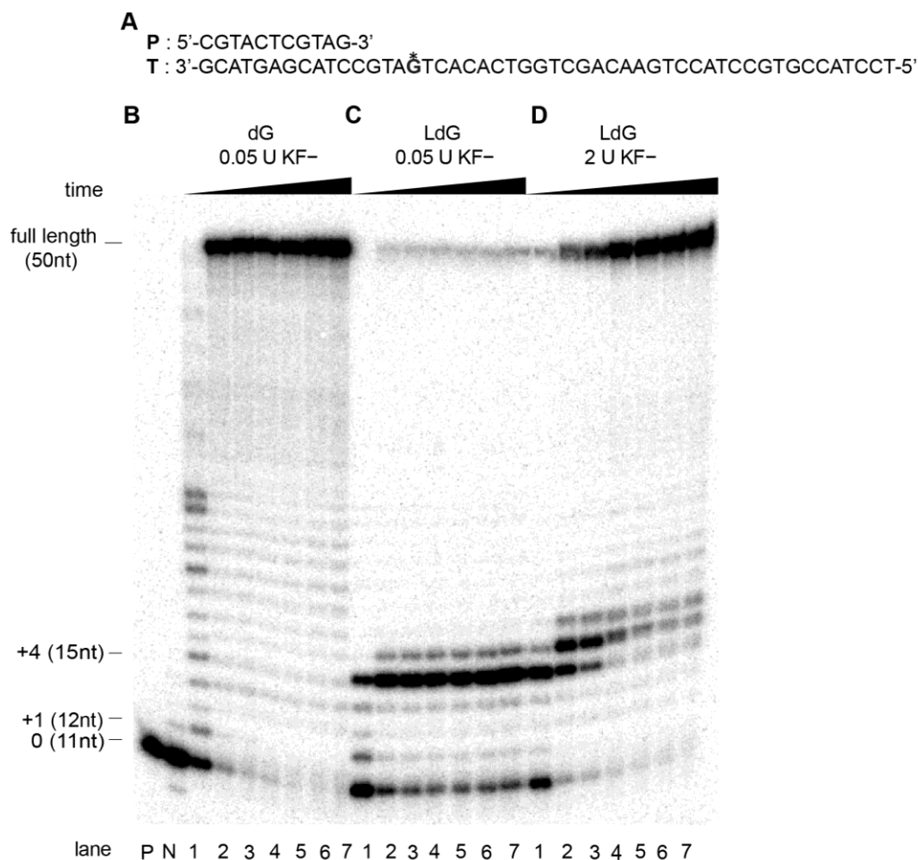
Figure S3. PAGE (20%, 7 M urea) of full length extension reactions using the \text{KF}^- with all dNTPs. A) Complete sequence of template, T ( \text{G}^* = \text{LdG} ) and primer, P; B) unmodified template (dG) with 0.05 U of \text{KF}^- ; C) modified template (LdG) with 0.05 U of \text{KF}^- ; D) modified template (LdG) with 2 U of \text{KF}^- . Lane P, primer; lane N, negative reaction control (no dNTPs); lanes 1 to 7: primer extension reactions with 100 \mu\text{M} of each dNTPs in different time course from 0.5, 5, 10, 30, 60, 120, and 240 min. All the reactions were carried out at 37 °C in the polymerase buffer (50 mM NaCl, 10 mM Tris-HCl, 10 mM \text{MgCl}_2 , 1 mM DTT, pH 7.9).
