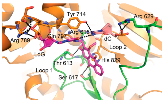
Figure 7. Active site orientation of the LdG adduct and pairing base dC in complex with the Bacillus fragment (BF). Polymerase is colored by domains (thumb in green, and finger in orange). The LdG adduct is shown in magenta, the hydrogen bonds between the atoms are represented in black dotted lines. The protein is rendered in cartoon, the atoms shown as sticks, and DNA as sticks along with filled rings. Key residues are labeled with numbers. Tyr 714 makes an H-bond with dC at a distance of 2.75 Å. Arg 629 and Arg 789 form an H-bond with LdG and dC, respectively, at a distance of ~2.73 Å. Ser 671 forms an H-bond with the carbonyl oxygen atom in the LdG at a distance of 2.63 Å. His 829 stacks on the polycyclic aromatic ring of LdG with a 3.0 Å distance. The W–C H-bond distance between LdG and dC is 3.1 Å. The conformer shown here is the averaged structure depicted in Figure 6C.
