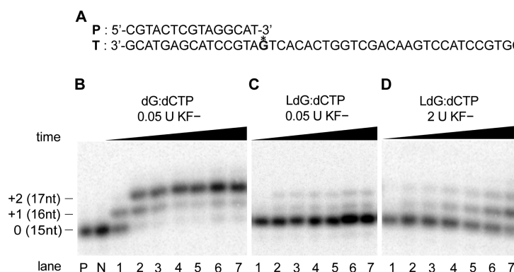
Figure 2. PAGE (20%, 7 M urea) of single nucleotide incorporation assay using \text{KF}^- . (A) Complete sequence of the template, T ( \text{G}^* = \text{LdG} ) and the primer, P; (B) unmodified template (dG:dCTP) with 0.05 U of \text{KF}^- ; (C) modified template (LdG:dCTP) with 0.05 U of \text{KF}^- ; (D) modified template (LdG:dCTP) with 2 U of \text{KF}^- . Lane P, primer; lane N, negative reaction control (no dCTP); lanes 1 to 7, primer extension reactions with 100 \mu\text{M} dCTP in a different time course from 0.5, 5, 10, 30, 60, 120, and 240 min. All reactions were carried out at 37 ^\circ\text{C} in the polymerase buffer (50 mM NaCl, 10 mM Tris-HCl, 10 mM \text{MgCl}_2 , 1 mM DTT, pH 7.9).
