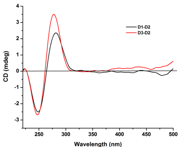
Figure S6. CD spectra for the unmodified ( D1-D2 ) and the LdG modified ( D3-D2 ) DNA duplexes (10 \mu M of each DNA strand in 100 mM NaCl, 20 mM sodium phosphate, 0.1 mM EDTA, pH 7.4). CD spectra show the characteristic peaks of B-form DNA. The enhanced CD intensity (280 nm) for the LdG modified DNA in comparison to the unmodified DNA may be attributed to the rigidly bound polycyclic aromatic adduct in the minor groove as revealed in our MD simulations. Similar CD spectrum is also observed for the N^2 -CH 2 (9-anthracenyl)-dG modified DNA. 4
