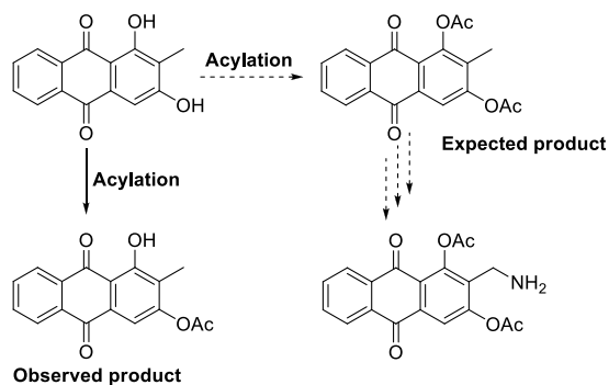
Figure S1. Synthetic strategy utilized for the 2-(aminomethyl)-1,3-diacetoxyanthraquinone
