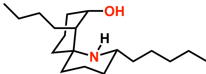
Perhydrohistrionicotoxin
