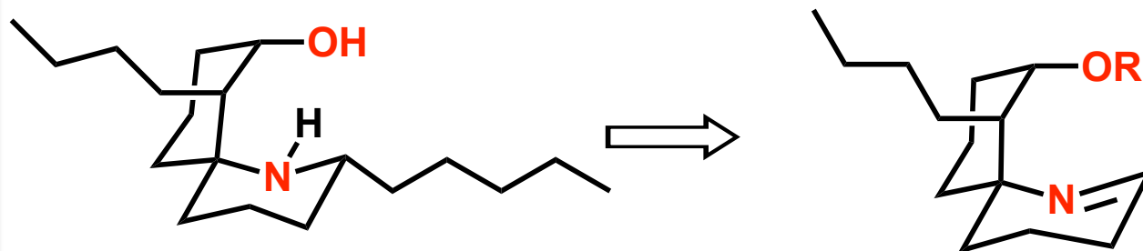
Perhydrohistrionicotoxin
