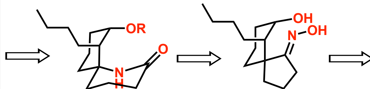
Perhydrohistrionicotoxin
