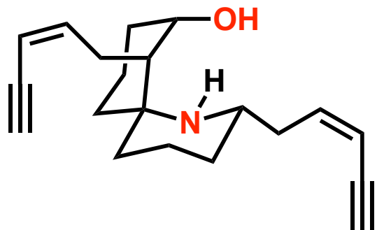
Histrionicotoxin
